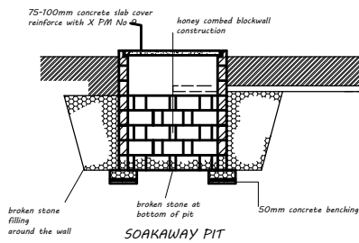
SOAKAWAY PIT
