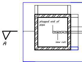
SOAKAWAY PIT
