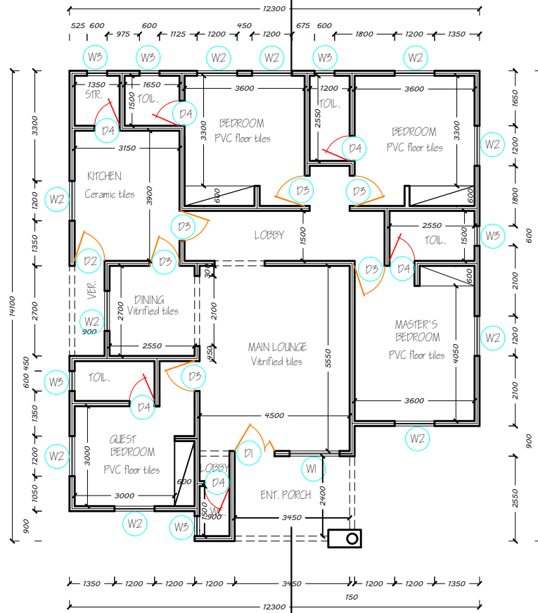
FLOOR PLAN
