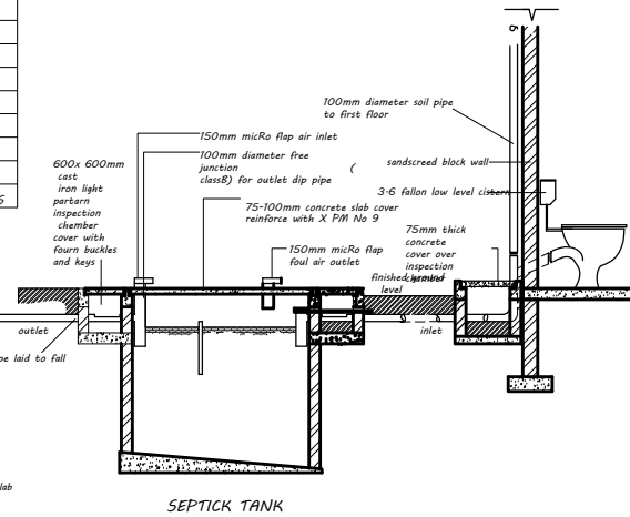
SEPTICK TANK
